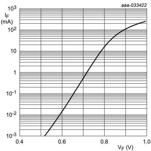
Fig. 2. Forward current as a function of forward voltage; typical values (BZX8850S-B/C1V8-Q)
