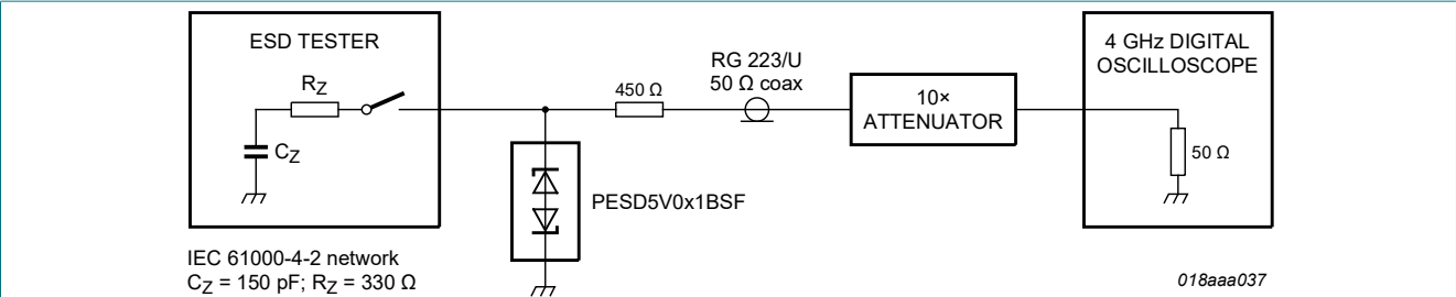
Fig. 5. ESD clamping test setup
