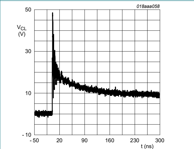
Fig. 8. Clamped +8 kV pulse waveform (IEC 61000-4-2 network)
