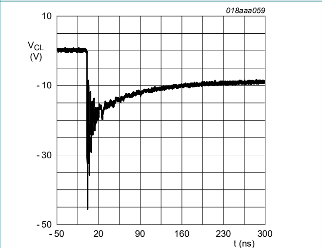
Fig. 9. Clamped -8 kV pulse waveform (IEC 61000-4-2 network)
