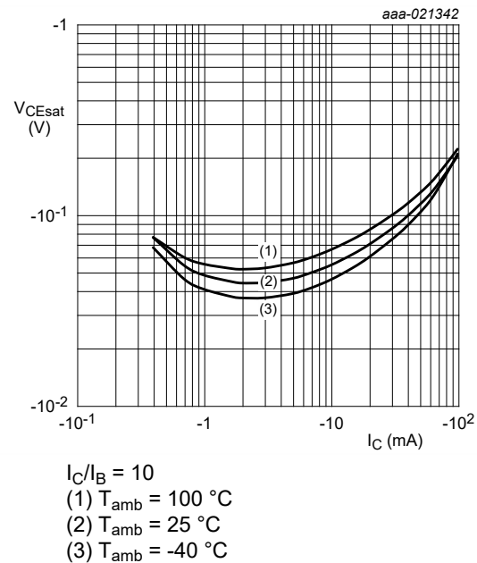
Fig. 15. PNP transistor: Collector-emitter saturation voltage as a function of collector current; typical values
