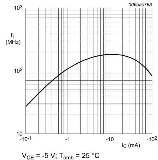
Fig. 17. PNP transistor: Transition frequency as a function of collector current; typical values of built-in transistor
