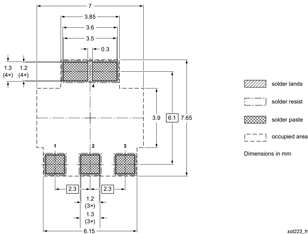
Fig. 3. Reflow soldering footprint for SC-73 (SOT223)
