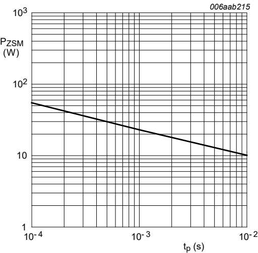
Fig. 1. Non-repetitive peak reverse power dissipation as a function of pulse duration; typical values
